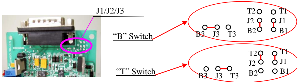
Figure 9. Socket Switch Connection of 9E-MFC
