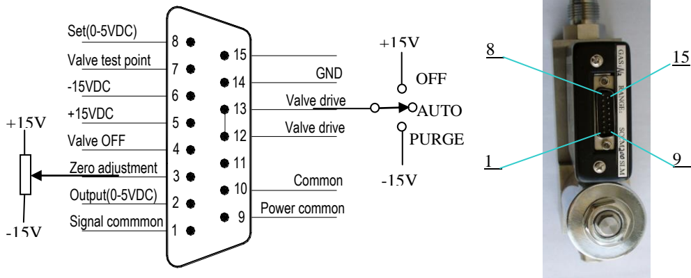
Figure 8. “B” Connection of D07-9E MFC
