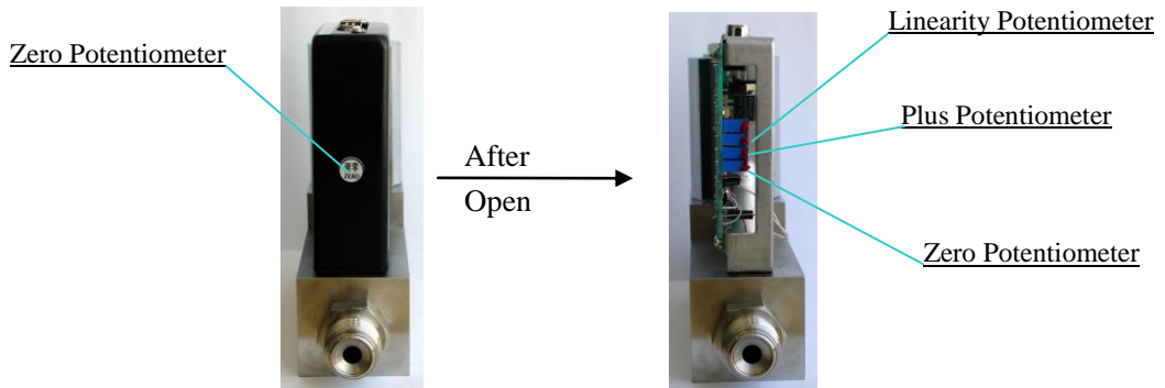
Figure 14. The Position of Potentiometer of 9E & 9EM
