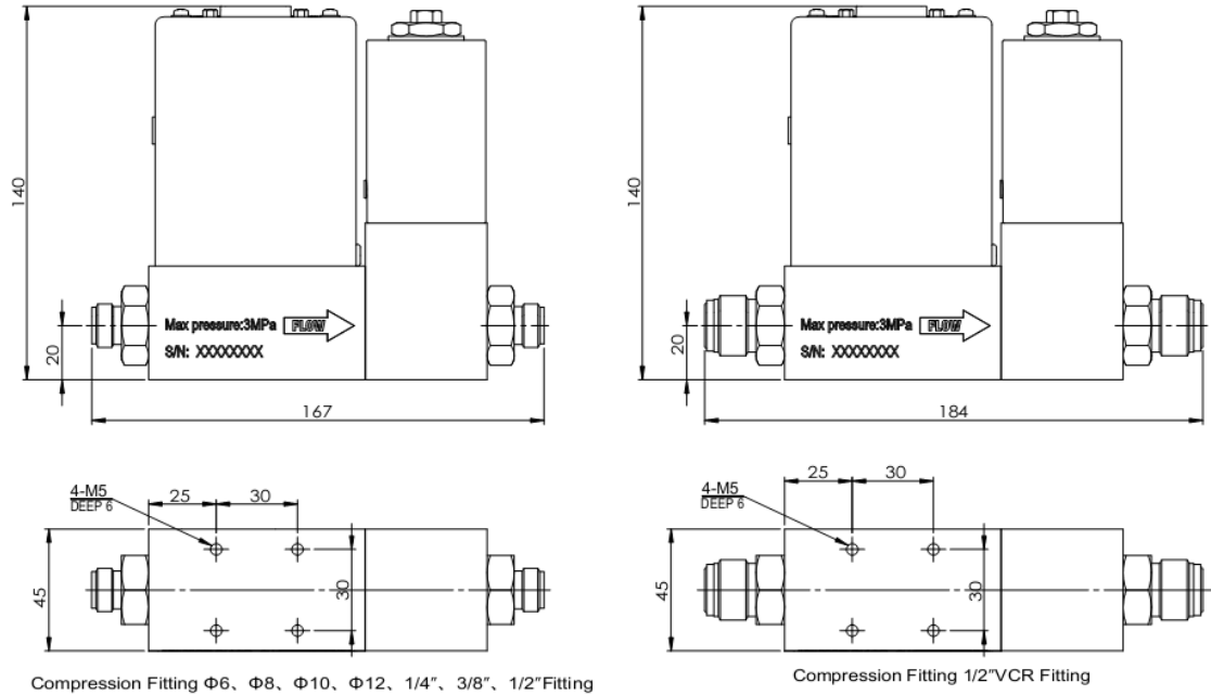
Figure 4. Dimension of D07-9E MFC
