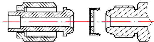
Figure 7. VCR Connector Installation
