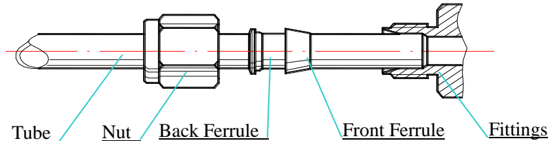
Figure 6. Compression Fitting Connector Installation
