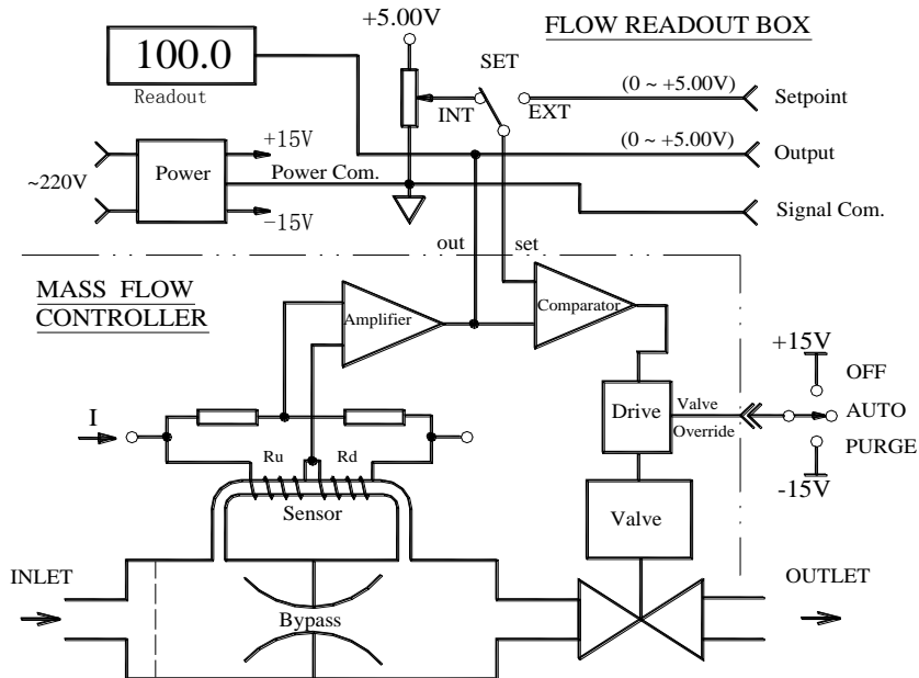
Figure3. Principle of MFC
