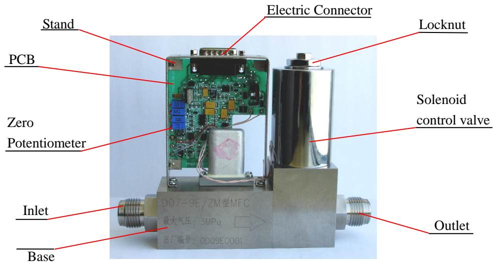
Figure 2. Structure of D07-9E MFC
