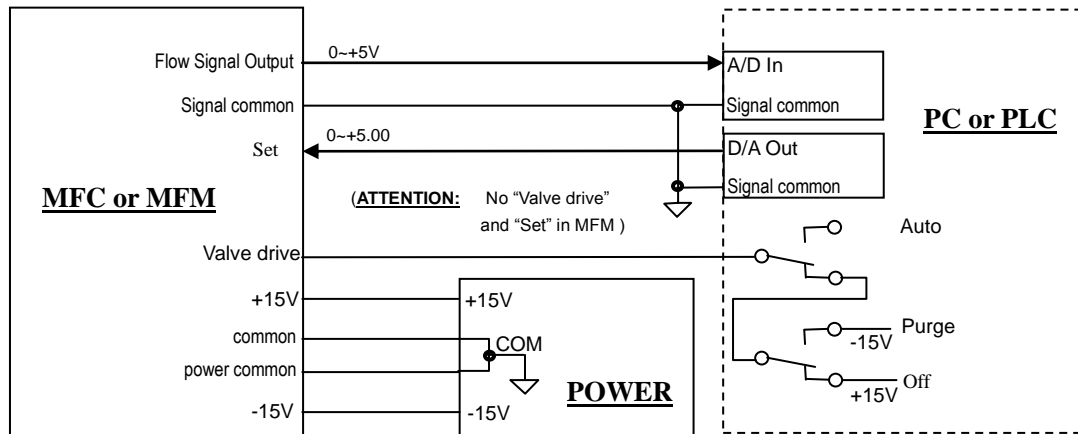
Figure 13. PC Directly Connection
