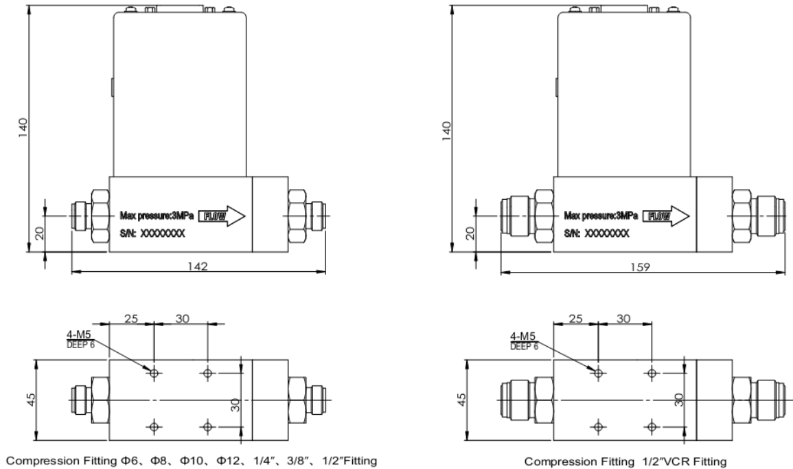
Figure 5. Dimension of D07-9EM MFM
